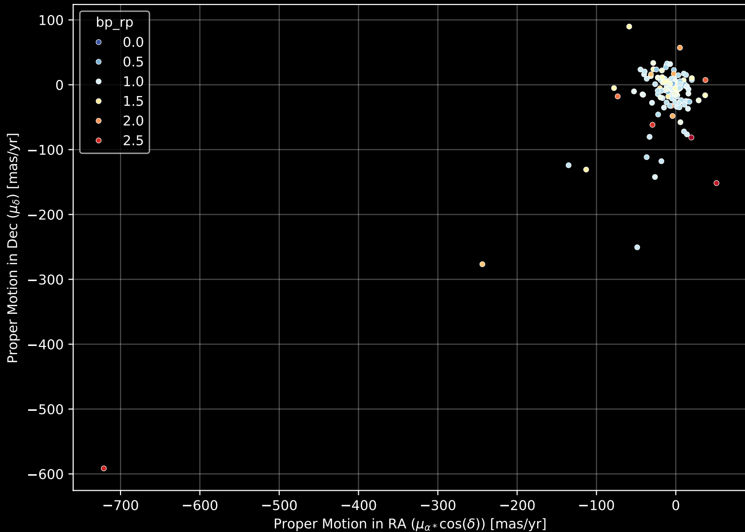
APOGEE DR17 Field: [045+42_MGA] Proper Motion Diagram (n= 165)
