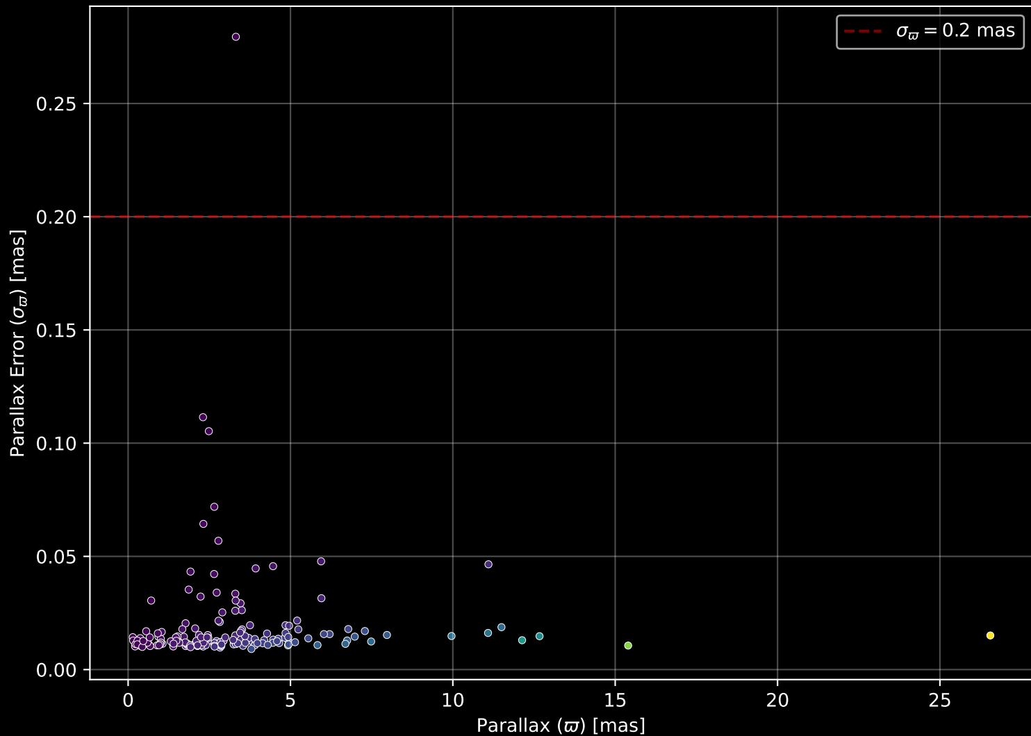
APOGEE DR17 Field: [045+42_MGA] Parallax Quality (n= 165)
