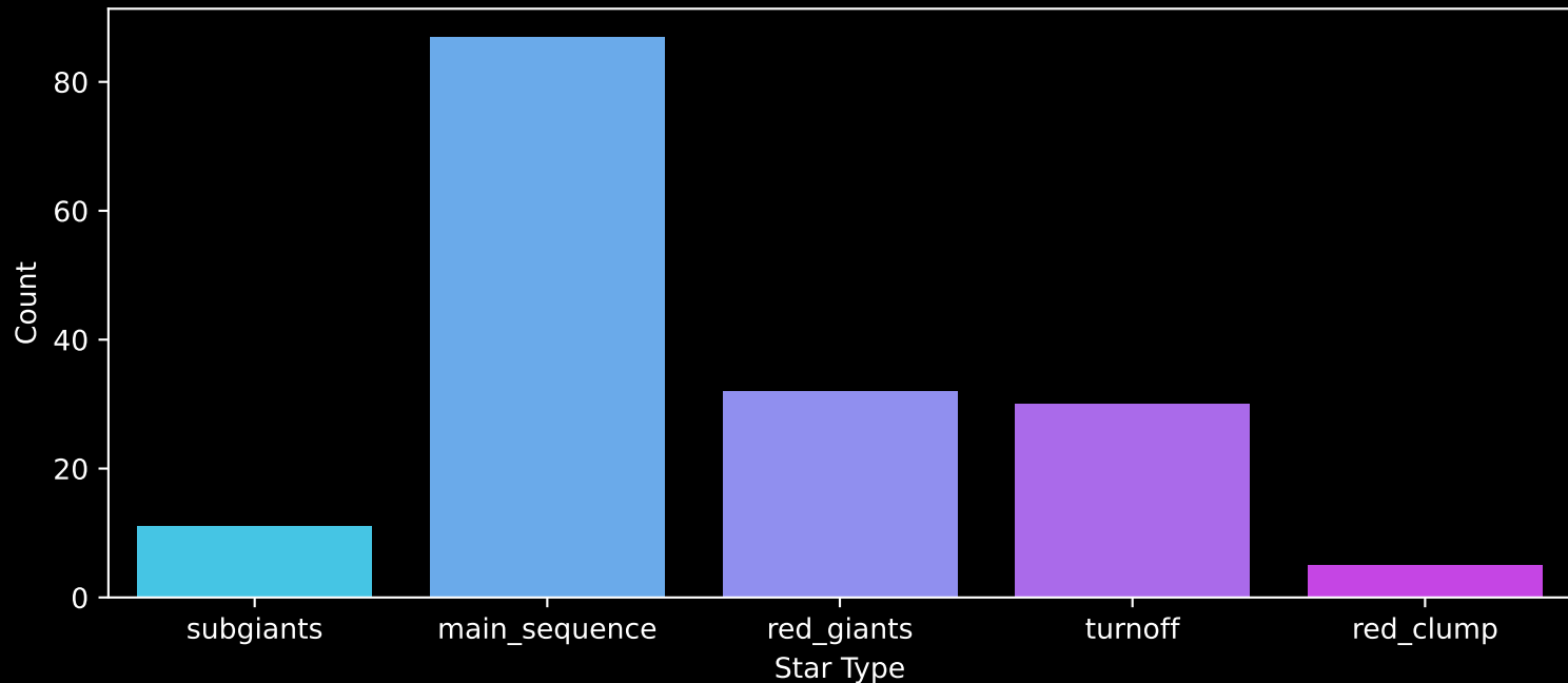
APOGEE DR17 Field: [045+42_MGA] Count plot of Star Type
