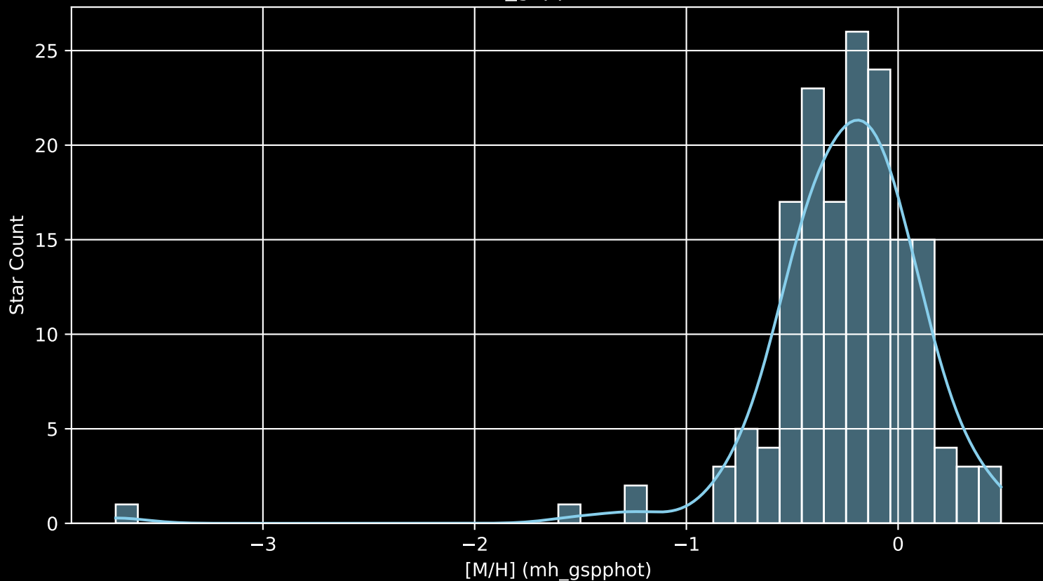
APOGEE DR17 Field: [045+42_MGA [M/H] (mh_gspphot) (n= 163)
