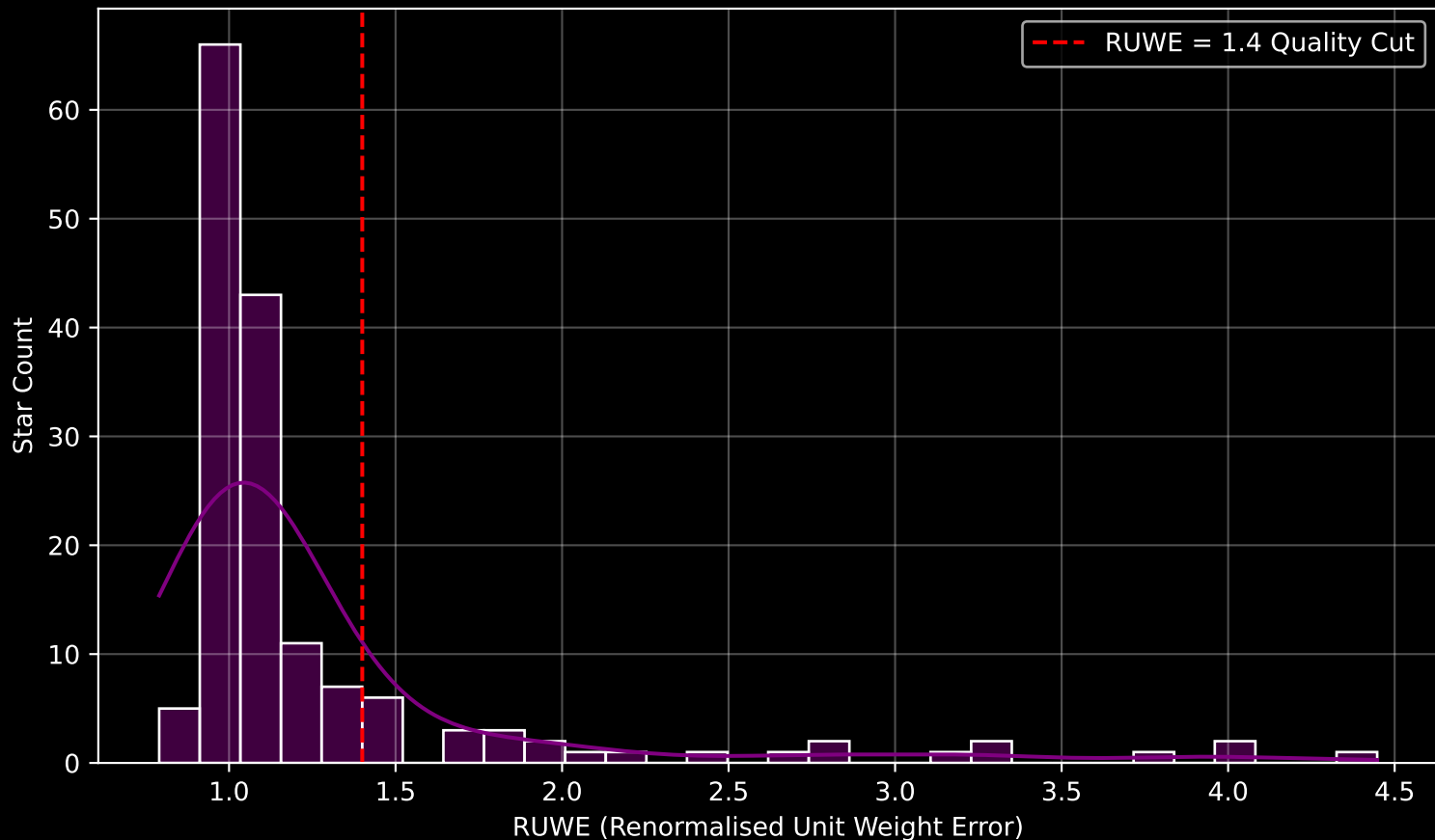
GAPOGEE DR17 Field [045+42_MGA] RUWE Distribution (n= 159)
