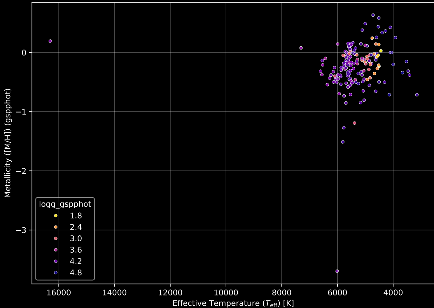
APOGEE DR17 Field: [045+42_MGA] Stellar Population Parameters (n= 165)
